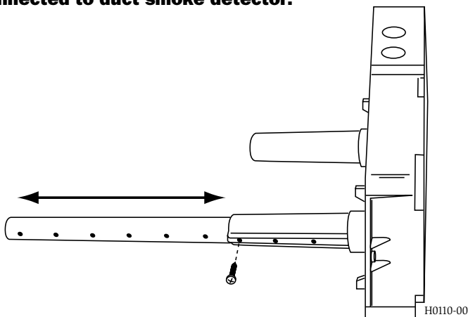
Figure 2. Plastic sampling tube connected to duct smoke detector:
