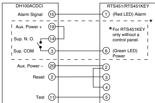
Figure 9. Wiring diagram for DH100ACDCI to RTS451KEY:
