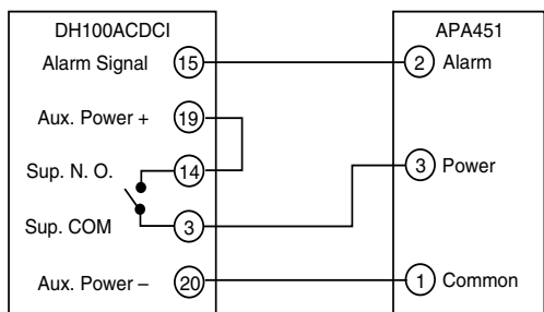
Figure 8. Wiring diagram for DH100ACDCI to APA451:
