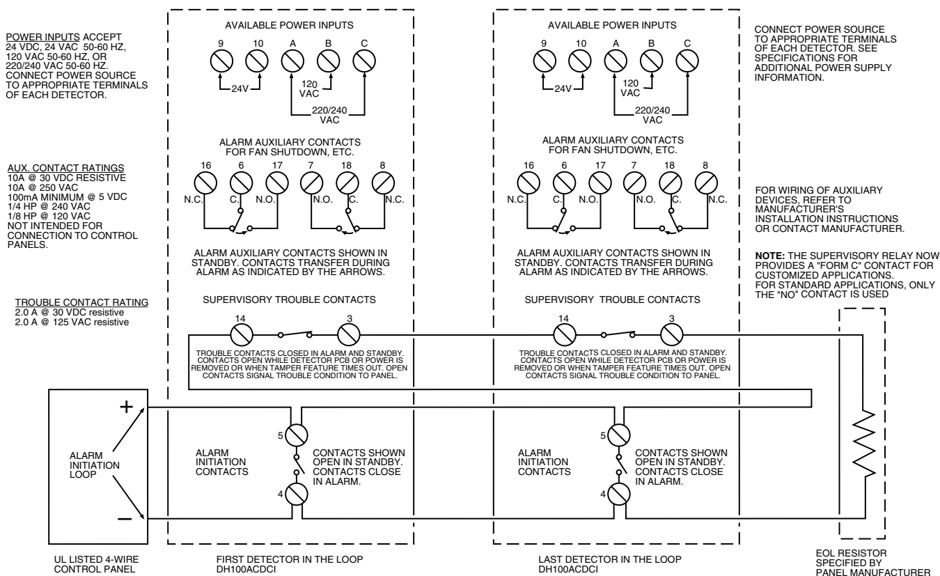
Figure 8. Wiring diagram for DH100ACDCI to APA451:
