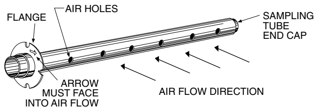
Figure 4. Air duct detector sampling tube:
