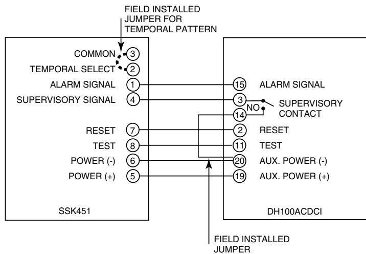
Figure 13. Testing detector alarm:
