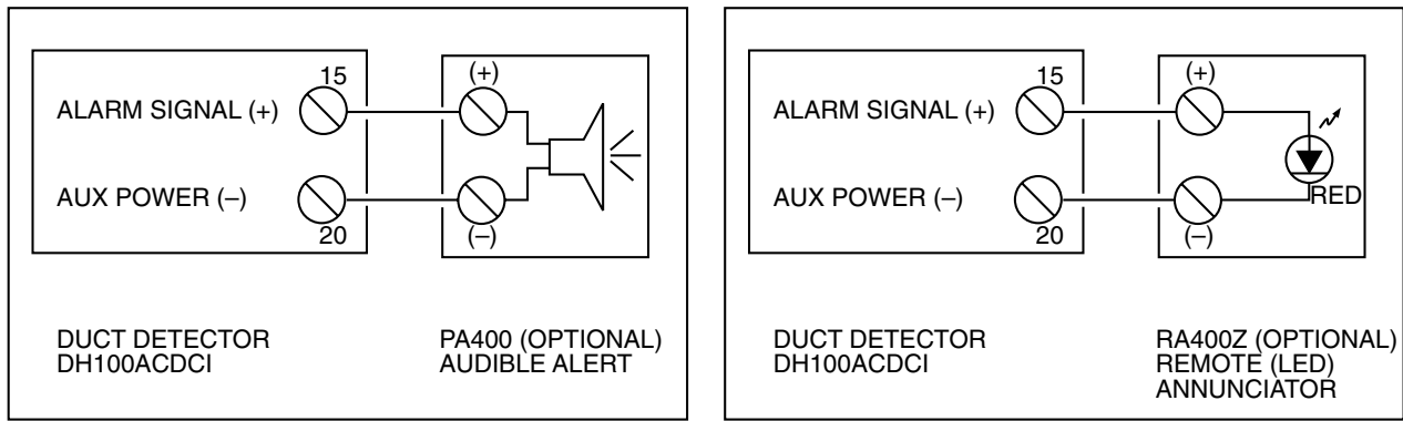
Figure 11. Wiring diagrams for optional accessories:
