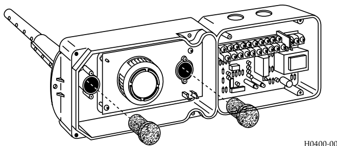
Figure 6. Sampling tube filter installation:
