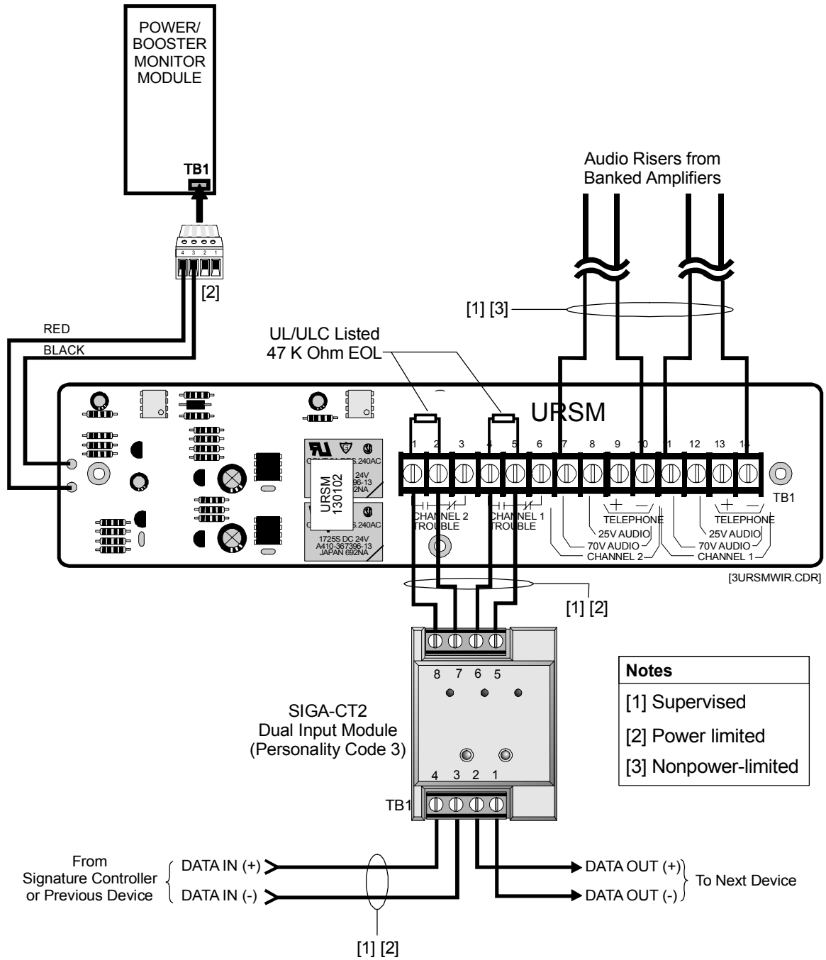
Figure 4-6: URSM wiring
