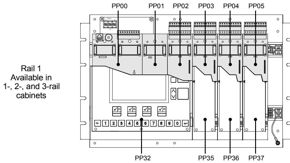
Figure A-5: LRM addresses when using a 3-LCDXL Main LCD Display
